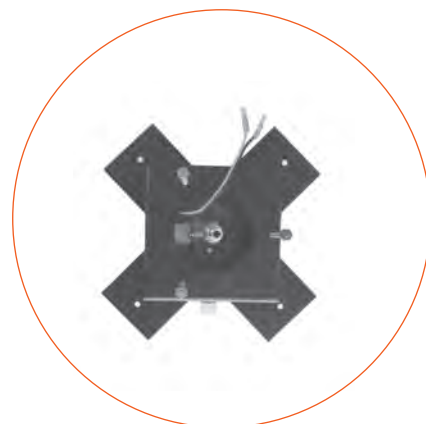
Cod. 9747 Corpo incasso / Built-in body per/for cod. 977/EL
