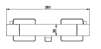
Cod. 43543CRPR Miscelatore termostatico doccia esterno Thermostatic external shower mixer
