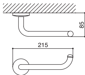
Cod. 04009CRPR Porta rotolo Toilet paper holder
