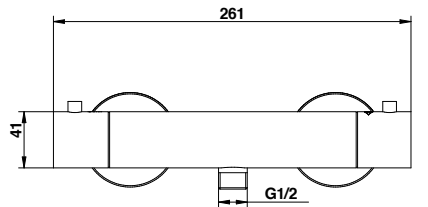
Cod. 32553CRPR Miscelatore termostatico doccia esterno Thermostatic external shower mixer
