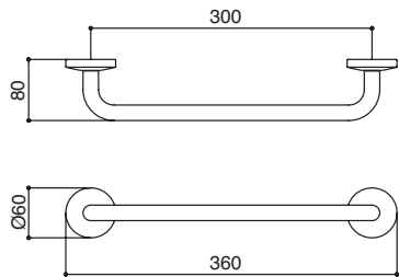
Cod. 04007/30/40/50/60CRPR Porta asciugamano cm. 30/40/50/60 30/40/50/60 cms. towel rail
