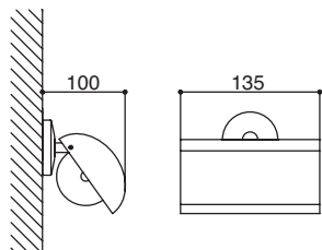
Cod. 04008CRPR Porta rotolo con ribalta Toilet paper holder with flap
